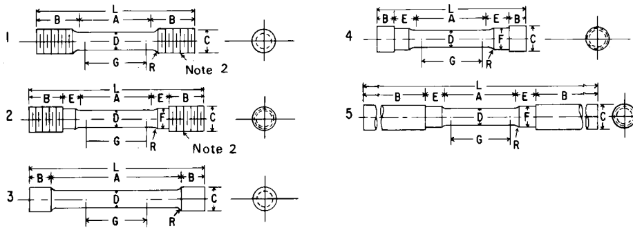
Dimensions, mm [in.] For Test Specimens with Gage Length Four times the Diameter [E8]
