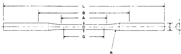
FIG. 17 Standard Tension Test Specimen for Malleable Iron
