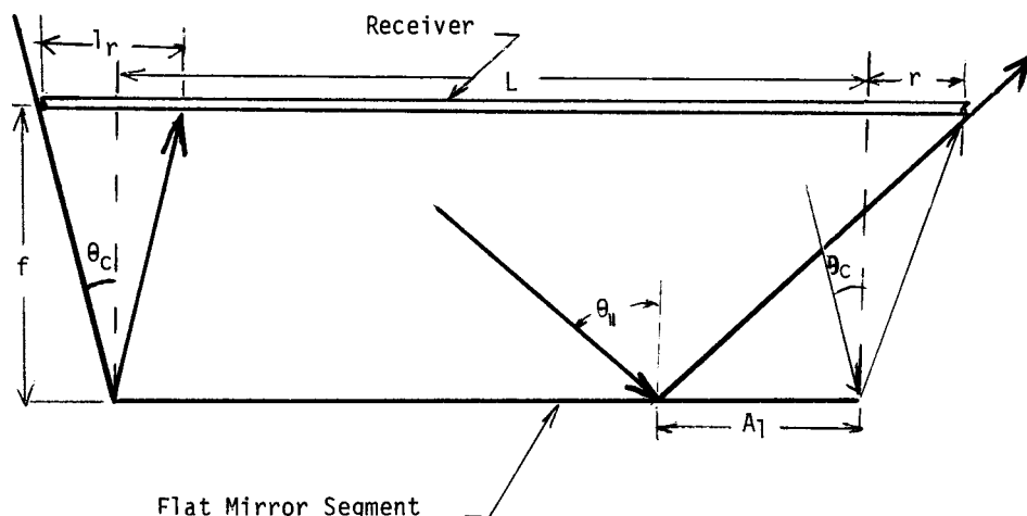
FIG. 1 End Effects in Cylindrical Array of Flat Segmented Mirrors
