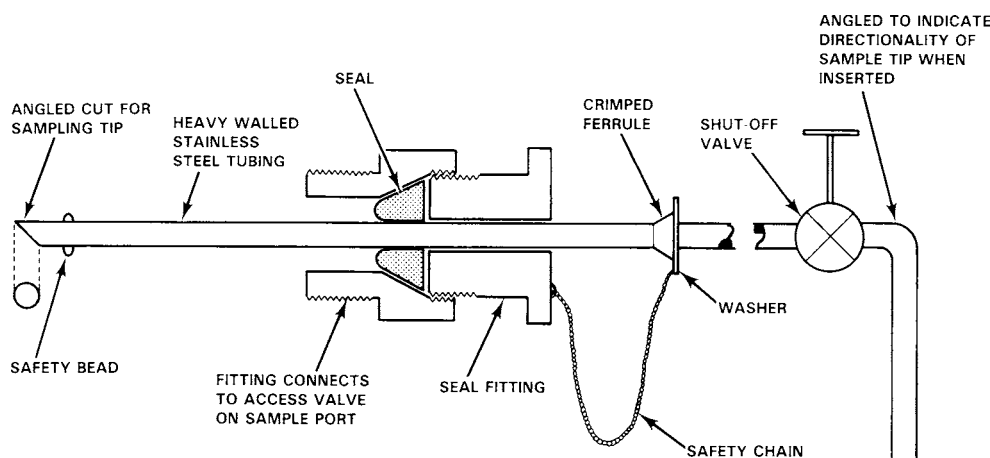
FIG. 2 Sample Probe
