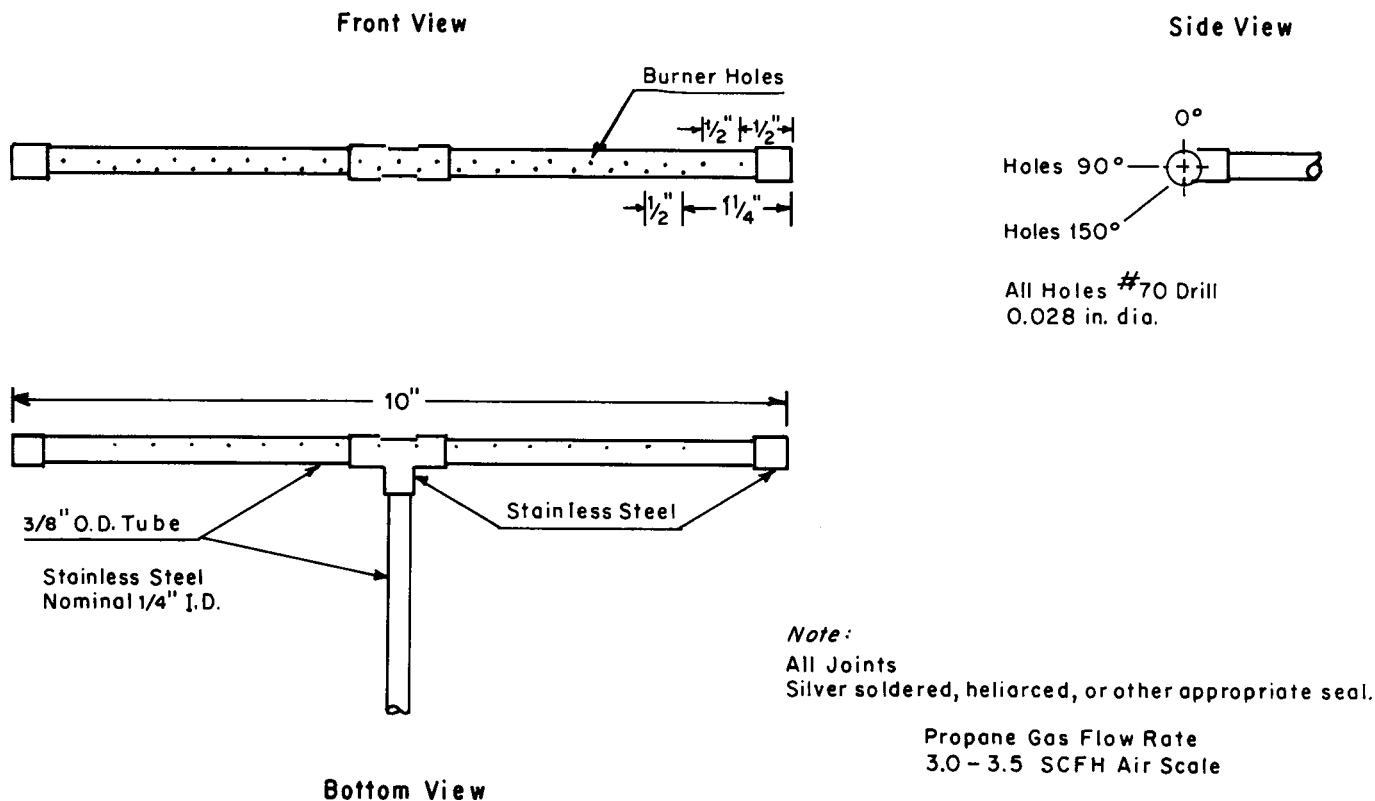
FIG. 6 Pilot Burner
