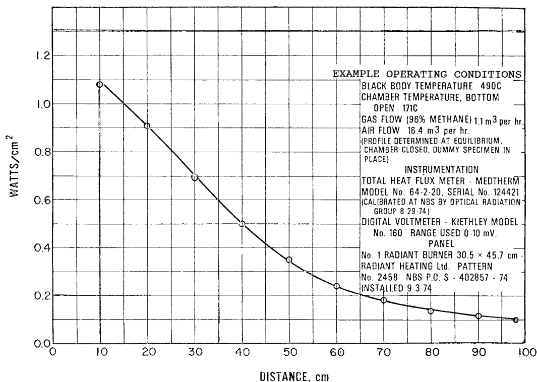
FIG. 8 Standard Radiant Heat Energy Flux Profile
