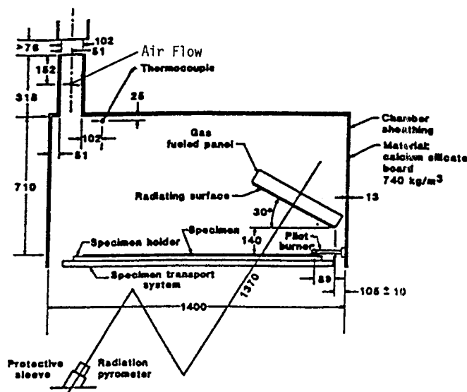
FIG. 1 Flooring Radiant Tester Schematic, Side Elevation
