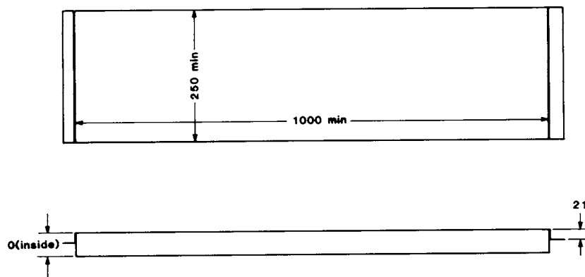
FIG. 5 Specimen Tray
