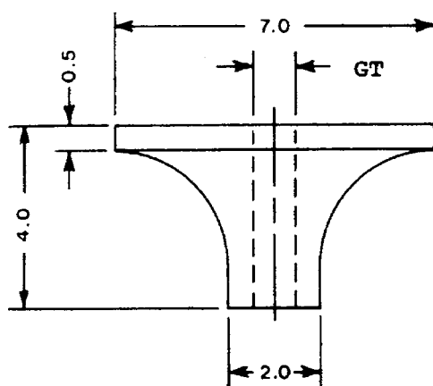
(a) Nielsen Shoe on Hsu Pencil Source
