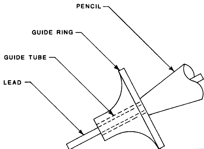
(a) Nielsen Shoe on Hsu Pencil Source
