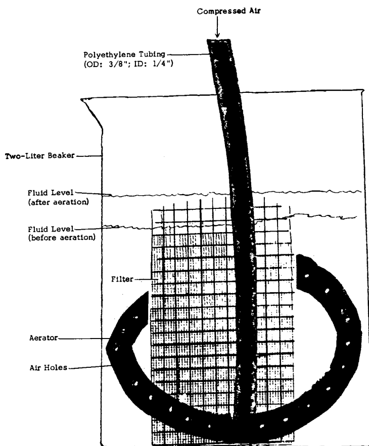
FIG. 1 Simulated Filter System
