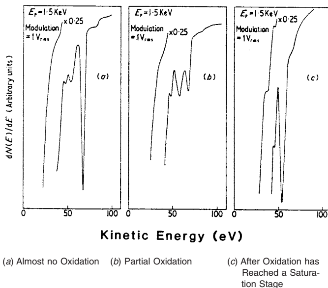
FIG. 3 Changes in the Aluminum LVV Auger spectrum as Oxygen is Absorbed on the Surface (Ref 15)
