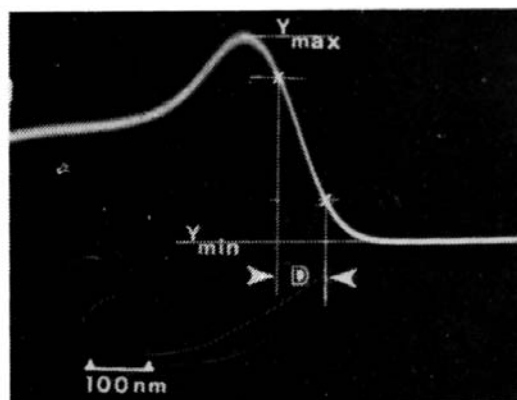
FIG. 2 Typical Waveform With 20 and 80 % Contrast Levels Illustrated
