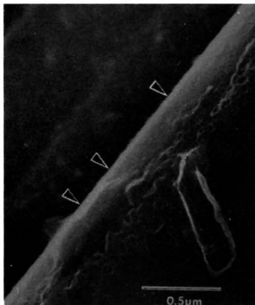
FIG. 1 Edge of Graphitized Natural Cellulose Fiber Used to Produce Line Traces (Fig. 3)
