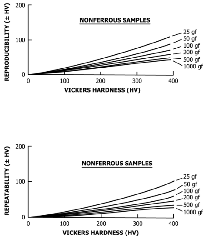
FIG. X3.3 Repeatability and Reproducibility Intervals in Terms of Vickers Hardness ( \pm ) for the Nonferrous Samples as a Function of Test Load and Specimen Hardness
