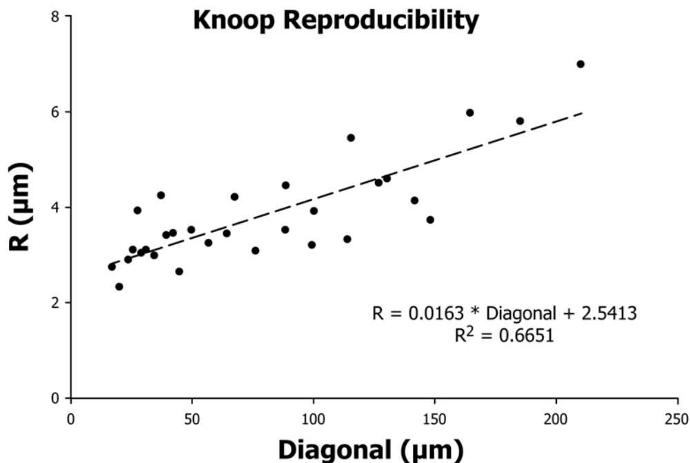
FIG. 4 The Relationship between Reproducibility ( R ) and Diagonal length ( d ) from Table 7 in μm units, for the Knoop Hardness Tests for Specimens B, C, D, E and T
