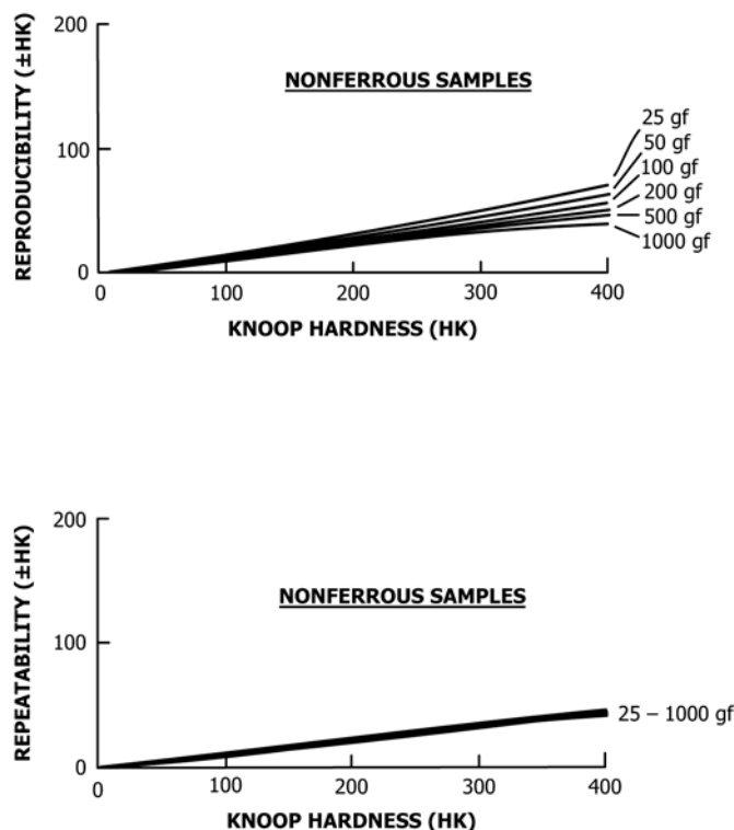
FIG. X3.4 Repeatability and Reproducibility Intervals in Terms of Knoop Hardness ( \pm ) for the Nonferrous Samples as a Function of Test Load and Specimen Hardness
