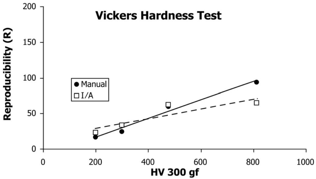
FIG. X4.4 Reproducibility of the Vickers 300 gf Manual and Automated Microindentation Hardness Tests
