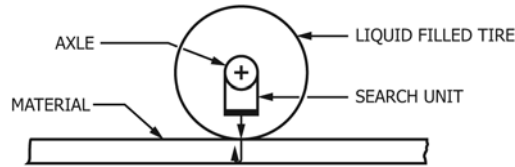
FIG. X2.2 Wheel Scanner
