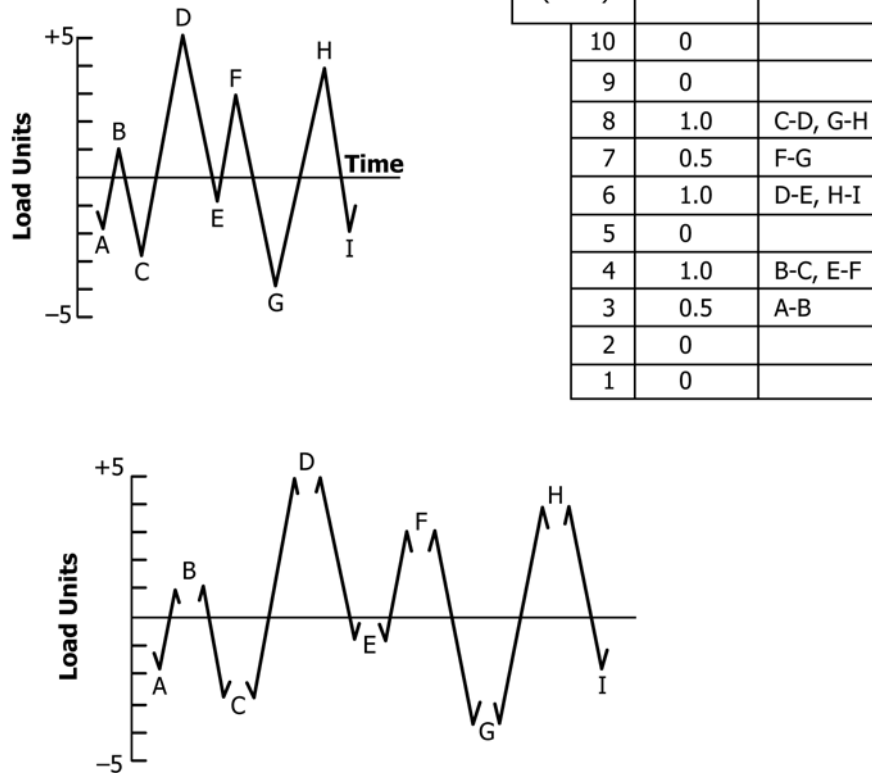
FIG. 4 Simple Range Counting Example—Both Positive and Negative Ranges Counted
