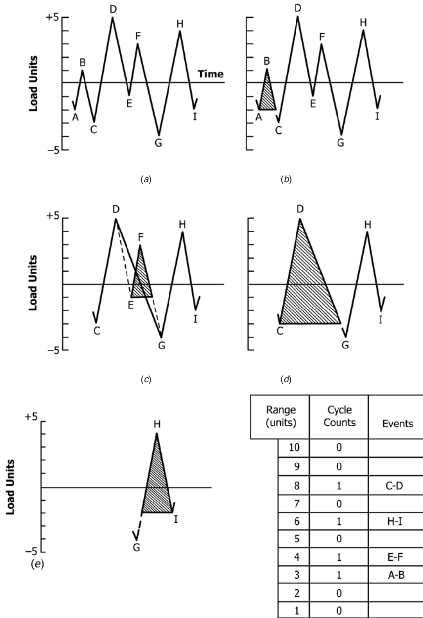
FIG. 5 Range-Pair Counting Example
