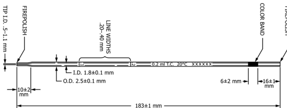
FIG. X1.1 Glass Micro Folin Pipet, Disposable
