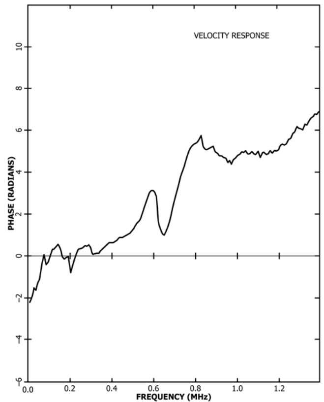
FIG. 14 Spectrum Phase Corresponding to the Spectrum Magnitude of Fig. 13
