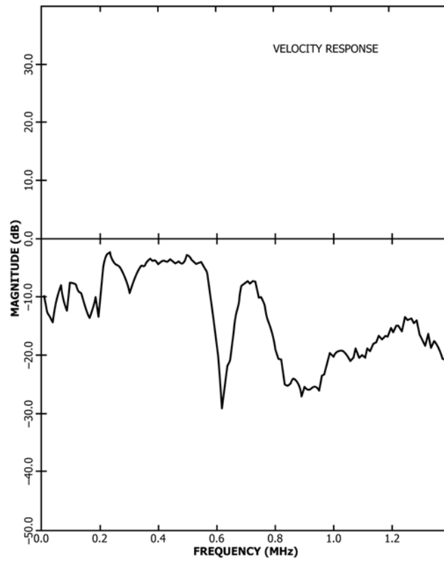
FIG. 15 Magnitude Response of the Unknown Transducer as Obtained by Division of the Ordinates of Fig. 13 by Those of Fig. 11
