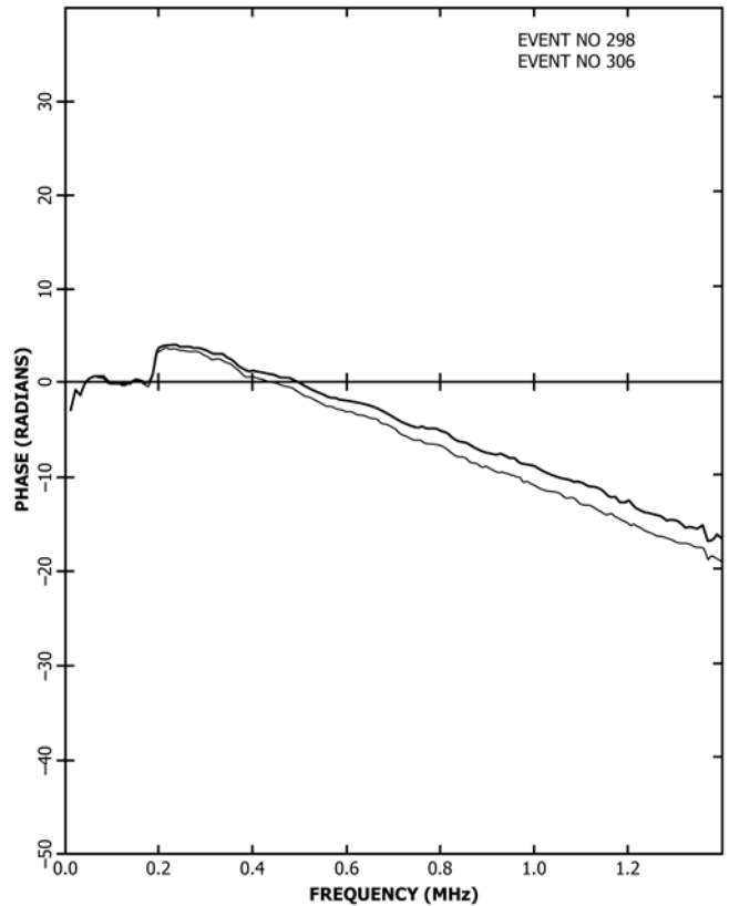
FIG. 8 Phase Responses Corresponding to the Magnitude Responses of Fig. 7
