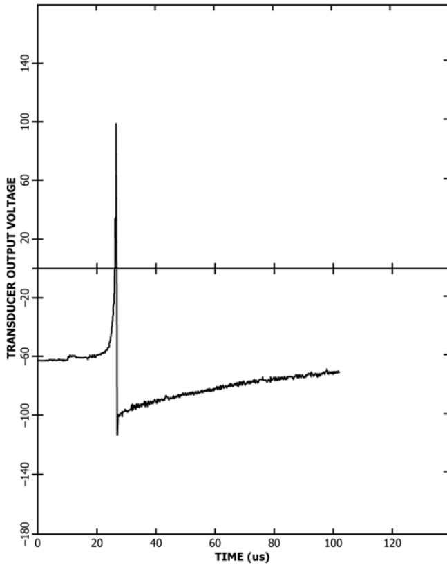
FIG. 9 A Typical Calibration—Voltage Versus Time Waveform from the Standard Transducer as Captured by the Transient Recorder (Note that the “shelf” value for the elasticity calculation of section 5.2.1 is located just after the negative going “overshoot”)
