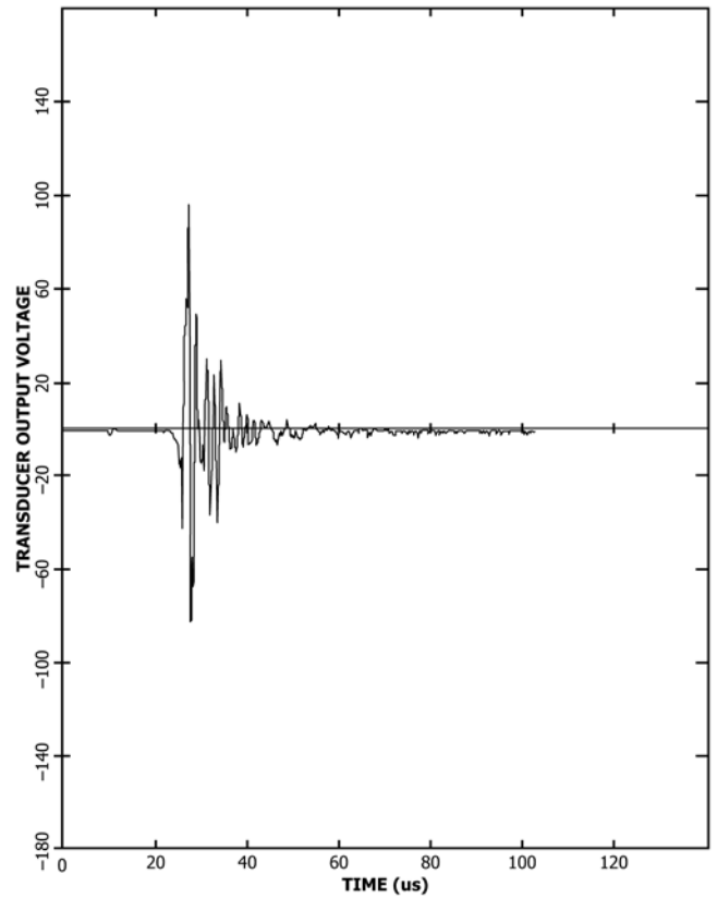
FIG. 10 The Same Calibration—Voltage Versus Time Waveform from the Unknown Transducer as Captured by the Transient Recorder
