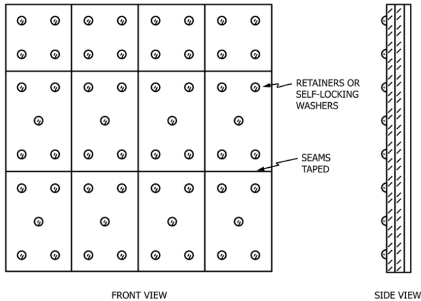
FIG. 3 (c) Acoustic Material Installation Details (continued)
