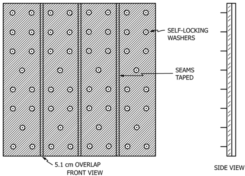
FIG. 3 (a) Acoustic Material Installation Details
