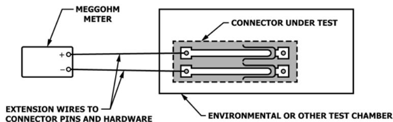
FIG. 5 Insulation Resistance Test
