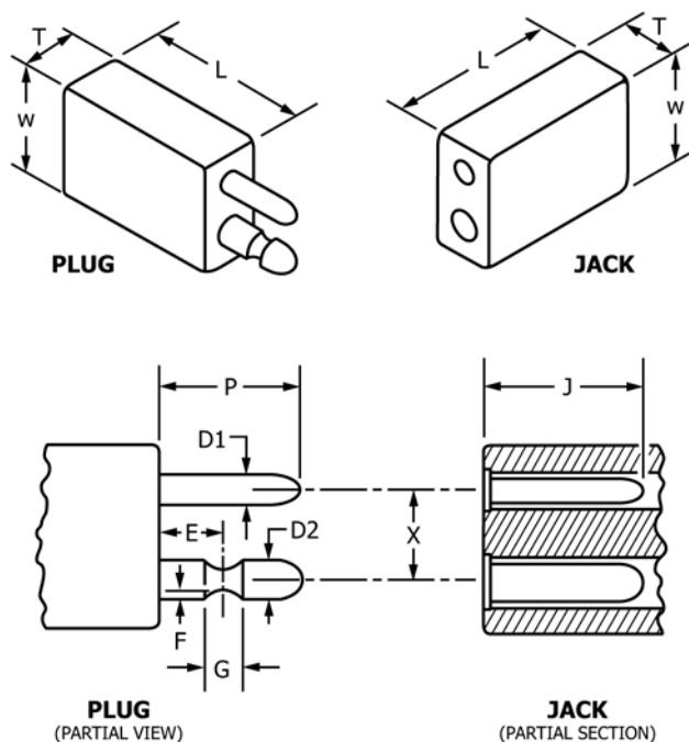
FIG. 1 Thermocouple Connector Dimensions, (see Table 1)
