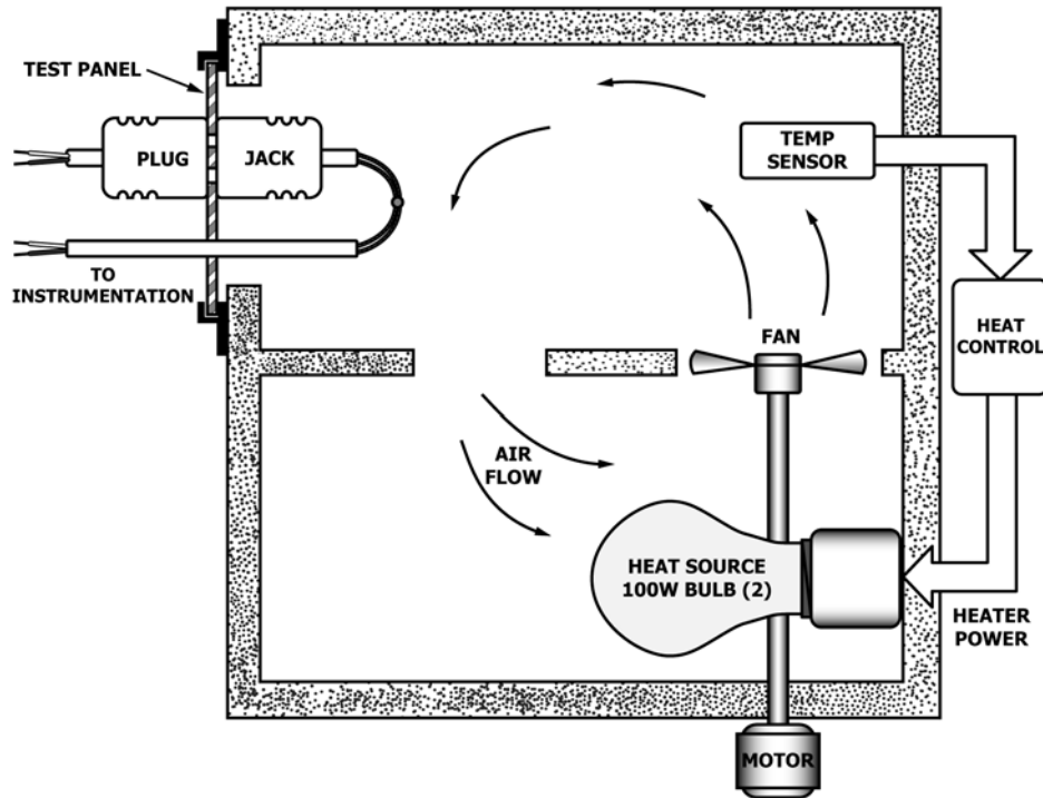
FIG. 3 General Arrangement for Thermal Gradient Test
