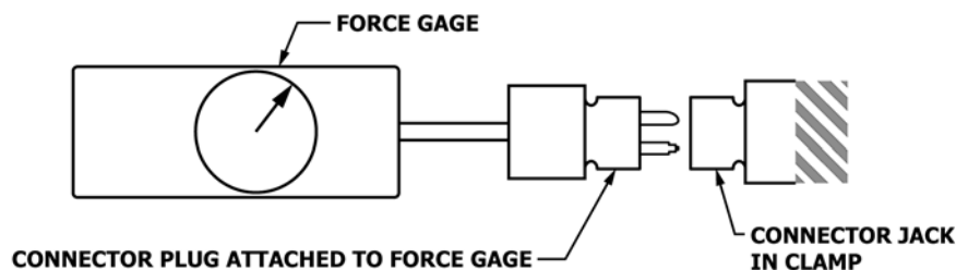
FIG. 6 Engagement/Disengagement Force Test
