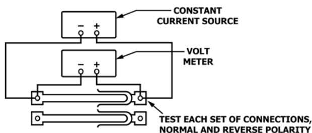
FIG. 2 Contact Resistance Test
