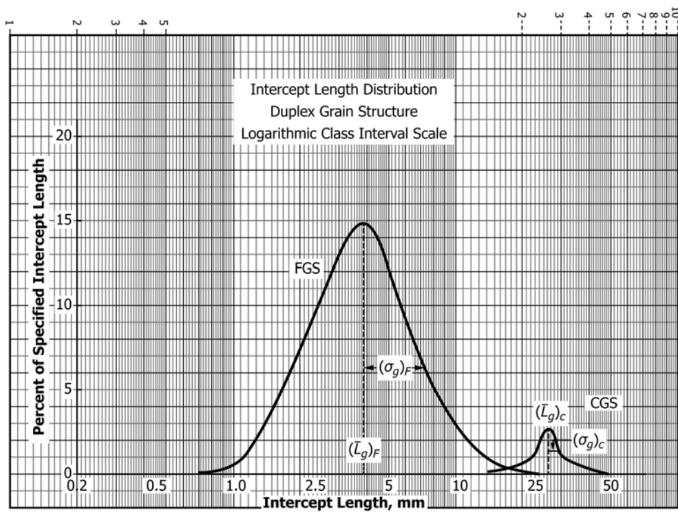
FIG. X2.4 Frequency Plot of Intercept Length Distribution (based on data from Table X2.1)
