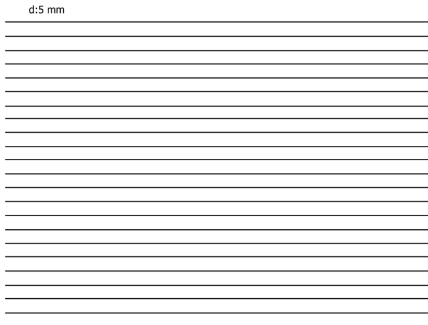
FIG. X2.1 Test Grid for Determining Statistical Distribution of Grain Intercept Lengths
