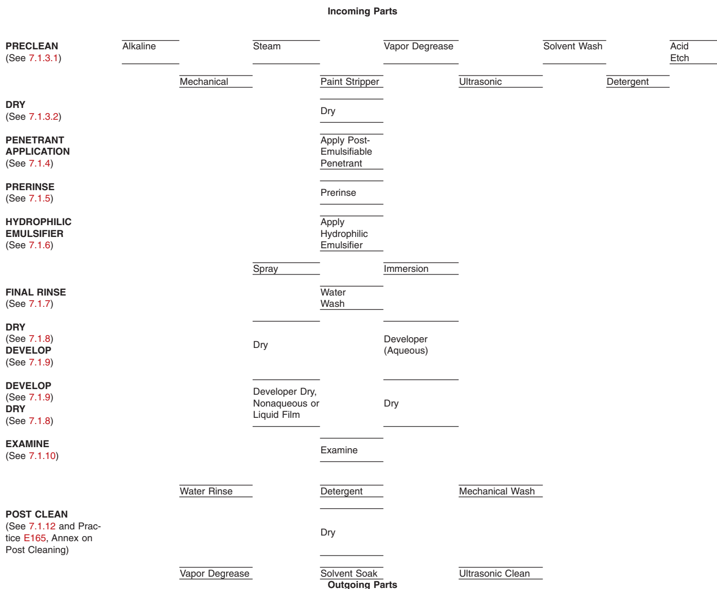
FIG. 1 General Procedure Flowsheet for Fluorescent Penetrant Examination Using the Water-Washable Process
