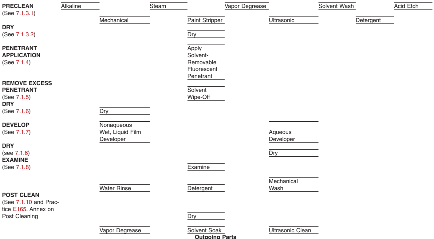
FIG. 1 Solvent-Removable Fluorescent Penetrant Examination General Procedure Flowsheet
