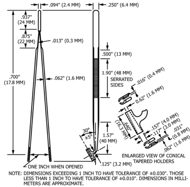
FIG. 20 Steel Forceps (Nickel Plated) with Conical Tapered Holders
