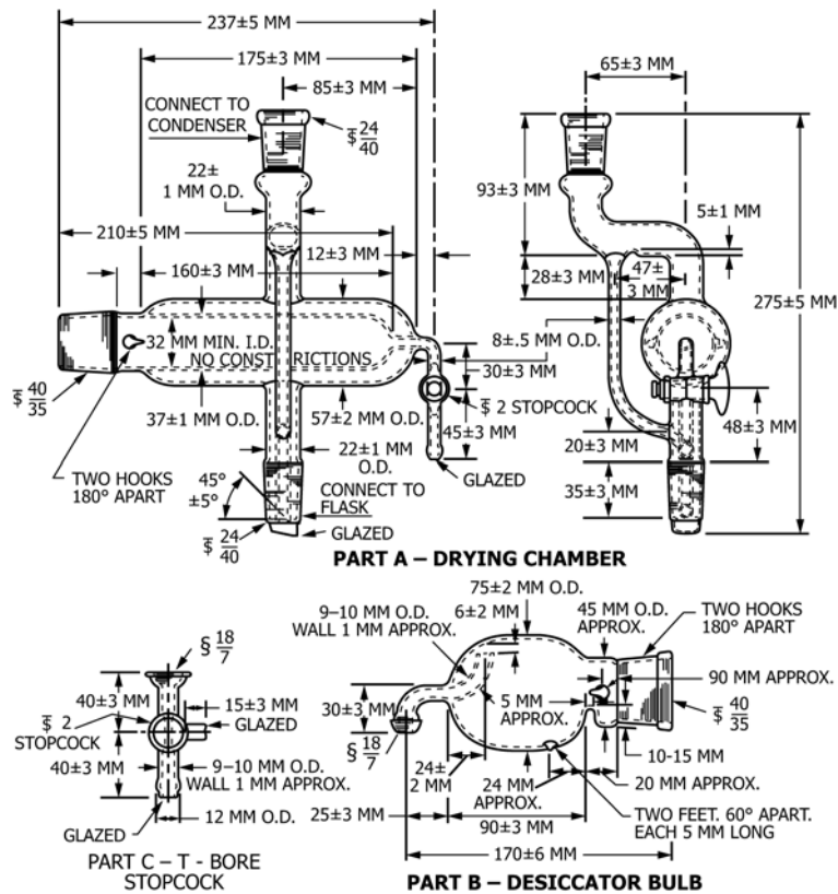
FIG. 27 Modified Abderhalden Drying Apparatus
