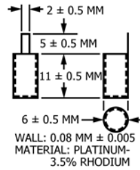
FIG. 11 Weighing Cup
