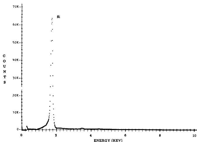
FIG. 2 EDX Analysis of Silicon Carbide Grinding Belt, 240-Grit
