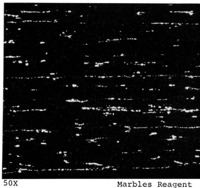
AISI M50 Bearing Steel
