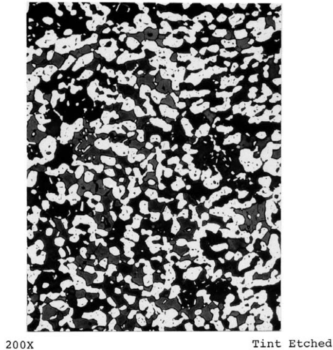
Wrought AISI 312 Stainless Steel
