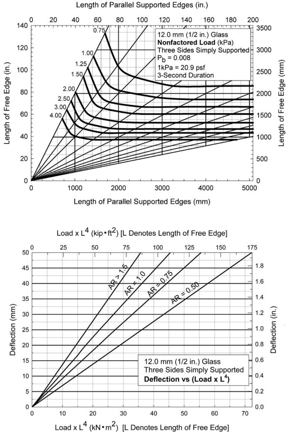
FIG. A1.22 (upper chart) Non-Factored Load Chart for 12.0 mm (1/2 in.) Glass with Three Sides Simply Supported (lower chart) Deflection Chart for 12.0 mm (1/2 in.) Glass with Three Sides Simply Supported
