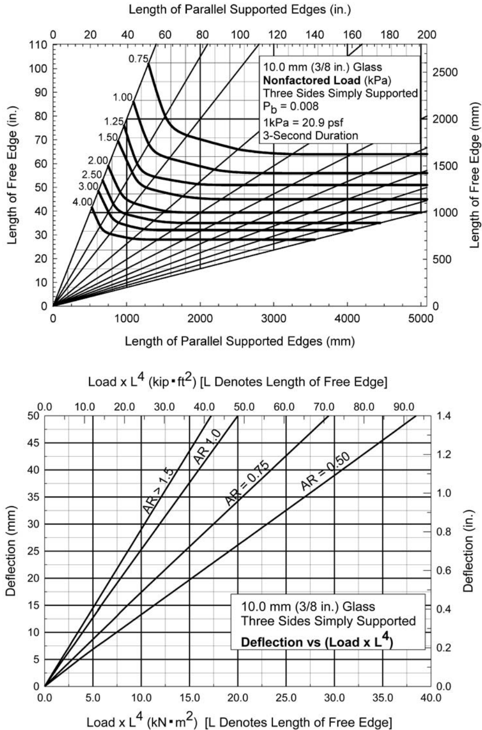
FIG. A1.21 (upper chart) Non-Factored Load Chart for 10.0 mm (3/8 in.) Glass with Three Sides Simply Supported (lower chart) Deflection Chart for 10.0 mm (3/8 in.) Glass with Three Sides Simply Supported
