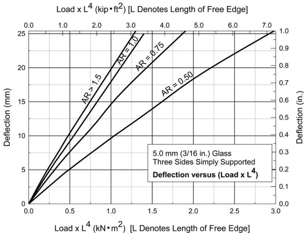
FIG. A1.18 (upper chart) Non-Factored Load Chart for 5.0 mm ( \frac{3}{16} in.) Glass with Three Sides Simply Supported (lower chart) Deflection Chart for 5.0 mm ( \frac{3}{16} in.) Glass with Three Sides Simply Supported
