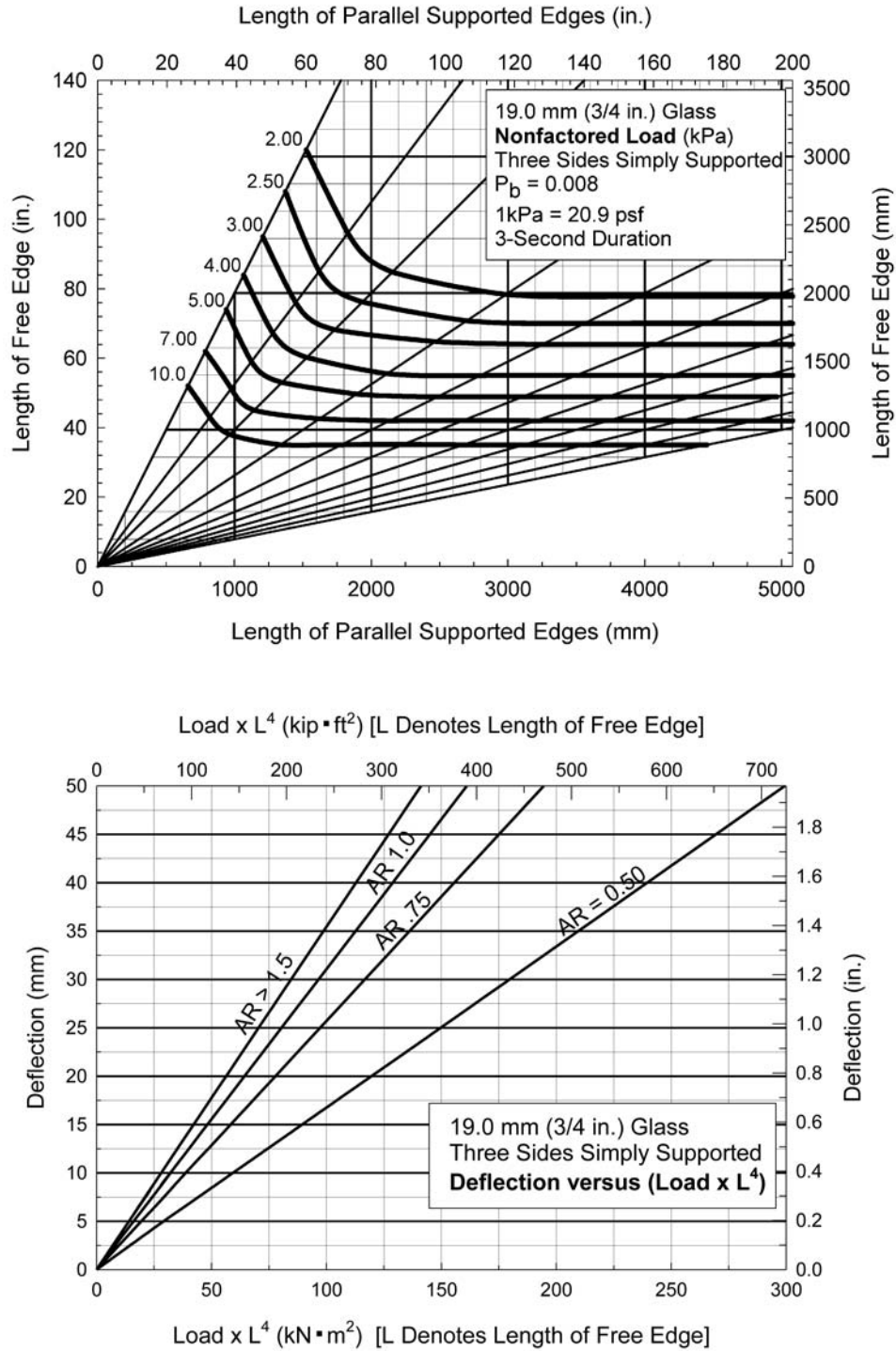
FIG. A1.24 (upper chart) Non-Factored Load Chart for 19.0 mm (3/4 in.) Glass with Three Sides Simply Supported (lower chart) Deflection Chart for 19.0 mm (3/4 in.) Glass with Three Sides Simply Supported
