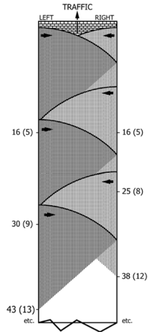
FIG. 1 Straightedge Positions
