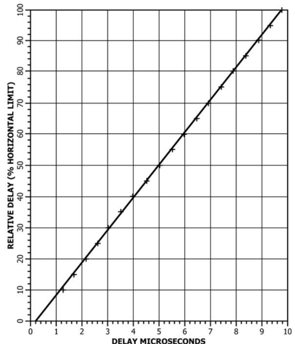
FIG. 9 Horizontal Linearity
