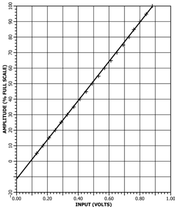
FIG. 7 Receiver Section Vertical Linearity
