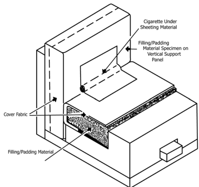
FIG. 7 Filling/Padding Component Test Method
