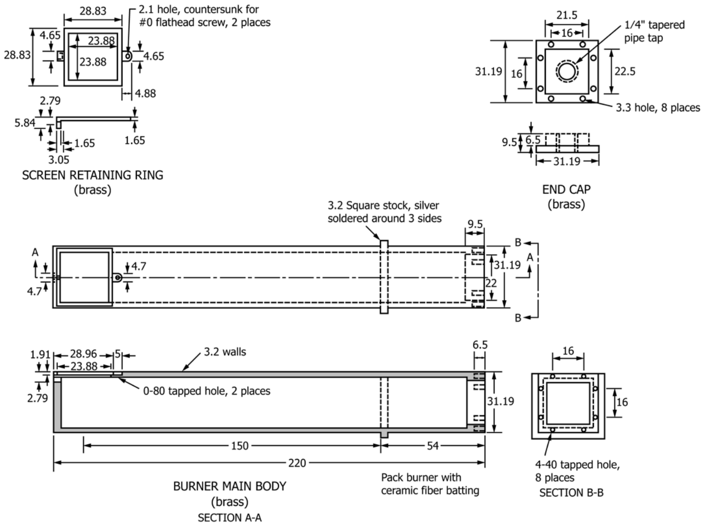
FIG. 11 Calibration Burner
