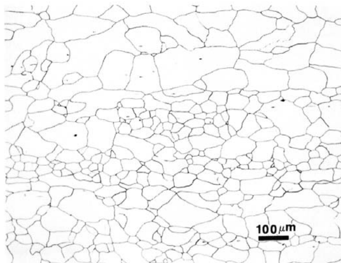
FIG. A2.14 Grain structure of the ferritic stainless steel specimen shown in Fig. A2.13 but after electrolytic etching with aqueous 60 % \text{HNO}_3 (Pt cathode, 1.2 V dc 15 s). Easily measured using a digitizing tablet and by automatic image analysis (after a minor amount of image editing).
