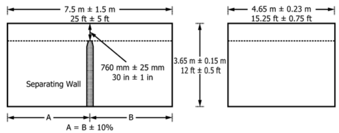
FIG. 1 General Dimensions of the Test Room
