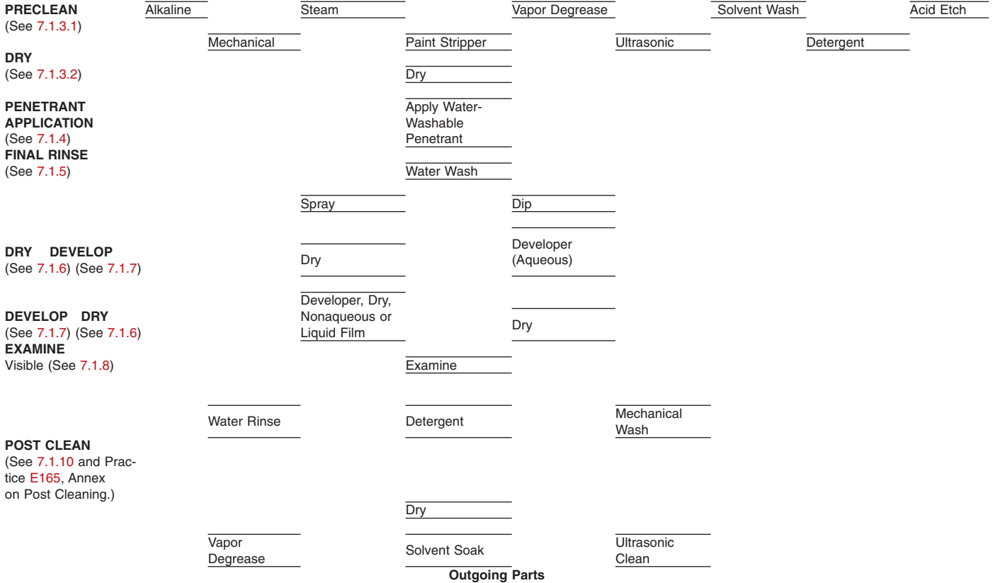
FIG. 1 General Procedure Flowsheet for Visible Penetrant Examination Using the Water-Washable Process
