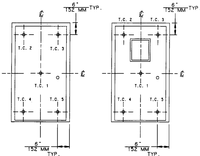
FIG. 6 Thermocouple Location: Entry Door
