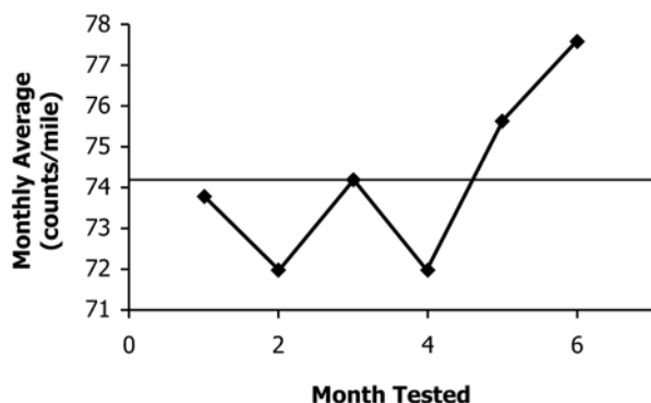
FIG. X3.2 Sample Mean and Range Control Charts [English Units]
