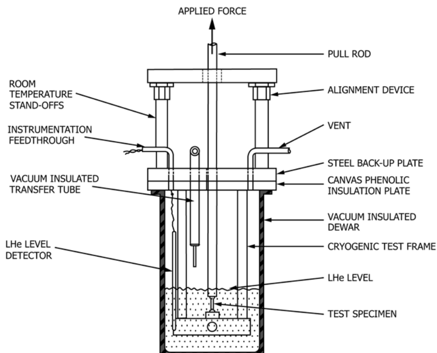
FIG. 1 Schematic Illustration of Typical Cryostat for Tension Testing at 4 K
