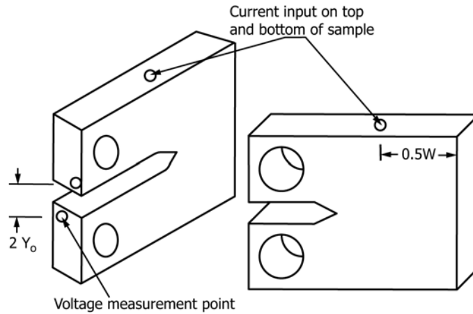
FIG. A1.6 Example Input Current and Voltage Lead Locations at the Back Face or the Starter Crack Front Placed on Either Side of the Specimen
