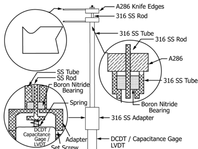
FIG. A1.4 Schematic of a Clip Gage Assembly for Measuring Force-Line (FLD) or Crack Mouth Opening (CMOD) Deflection in Different Geometries
