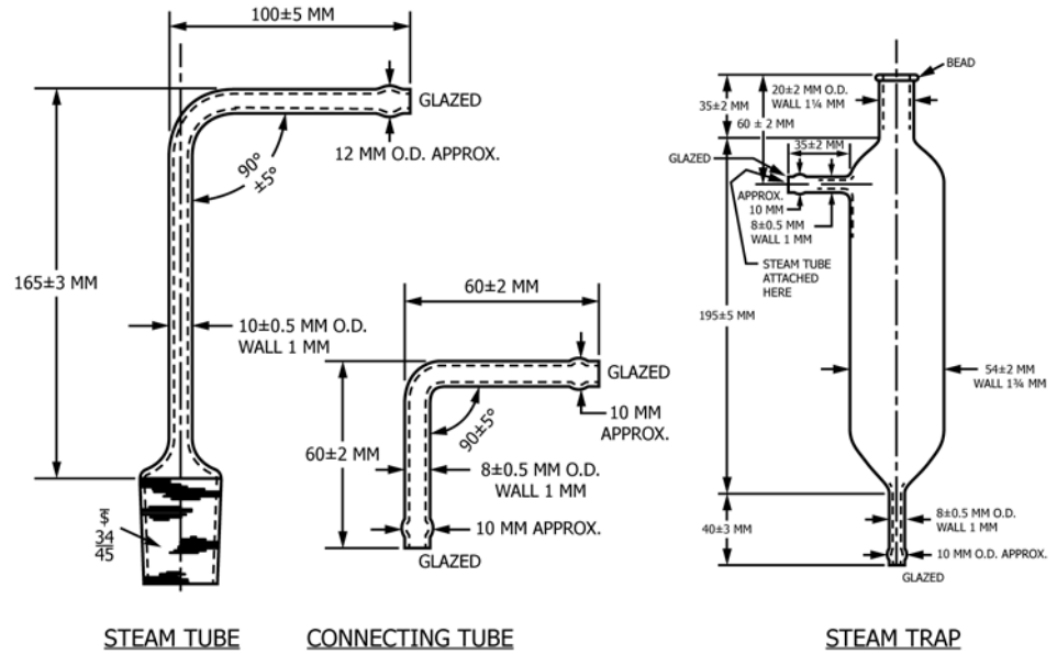
FIG. 9 Steam Tube, Steam Trap, and Connecting Tube
