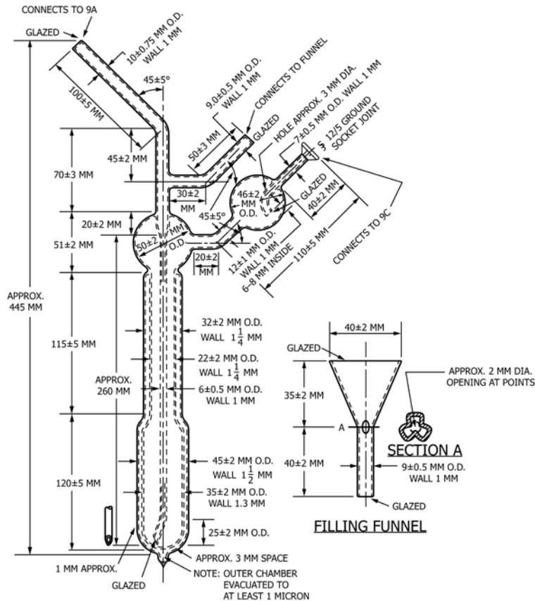
FIG. 10 Distillation Flask and Filling Funnel
