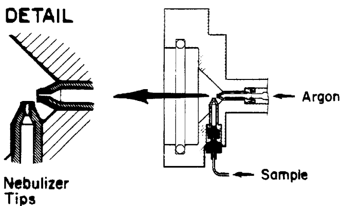
FIG. 4 Cross-Flow Nebulizer 4
