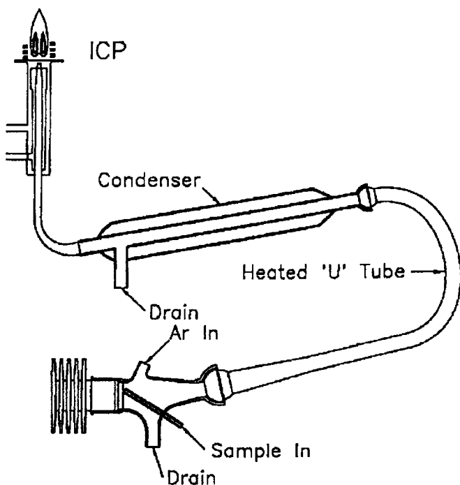
FIG. 10 Ultrasonic Nebulizer 5
