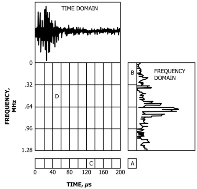
BLOCK "A" IS FOR THE TOTAL WAVEFORM OR SPECTRUM. BLOCK "B" IS FOR THE FREQUENCY INTERVAL 0 TO 0.3 MHz. BLOCK "C" IS FOR THE TIME INTERVAL 120 TO 140 μs. BLOCK "D" IS FOR THE INTERVAL 0.3 TO 0.6 MHz, 40 TO 60 μs.
