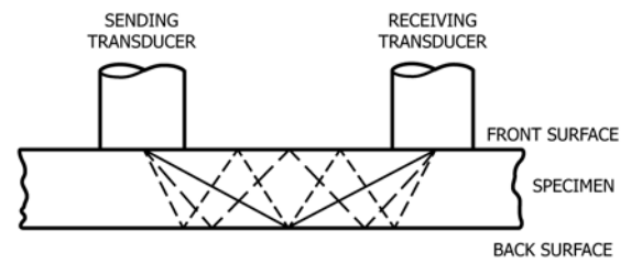
(A) FIRST, SECOND, AND THIRD ORDER LONGITUDINAL (P-WAVE) RAY PATHS.
