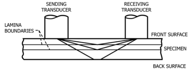
(B) FIRST ORDER LONGITUDINAL (P-WAVE) RAY PATHS IN LAMINATED SOLID.
