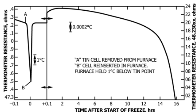
FIG. 4 Freezing Curve of a Sample of Highly Purified Tin
