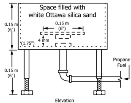
FIG. 12 Calibration Gas Burner
