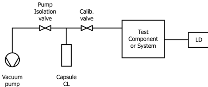
FIG. 4 Calibration Setups
