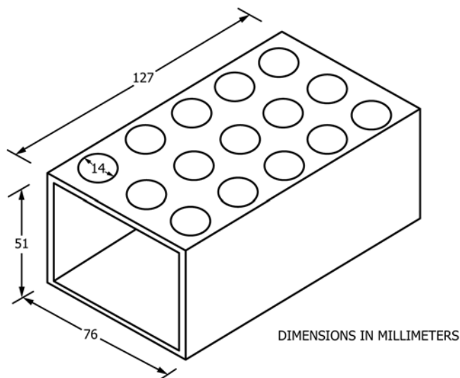
FIG. 7 Calibration Jig
