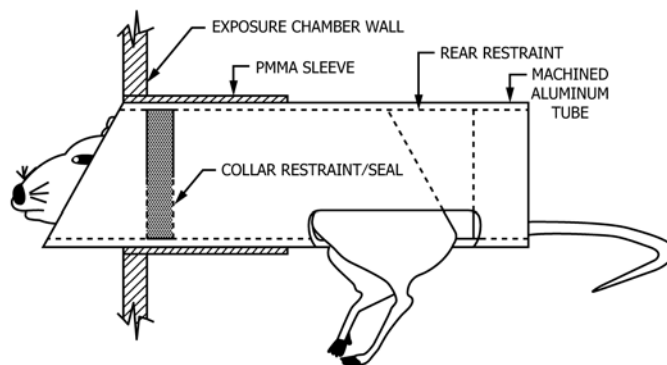
ANIMAL RESTRAINT
