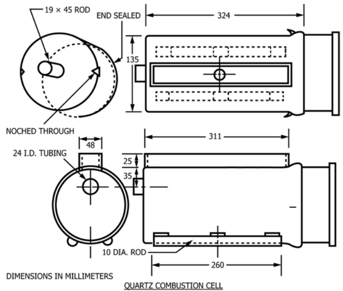
FIG. 6 Combustion Cell
