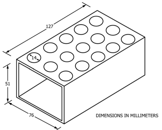
FIG. 7 Calibration Jig
