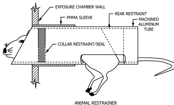
FIG. 10 Animal Restraint
