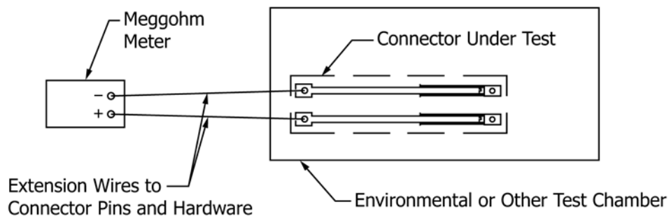
FIG. 5 Insulation Resistance Test
