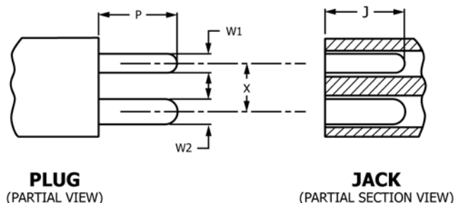
FIG. 1 Miniature Thermocouple Connector Dimensions (see Table 2)
