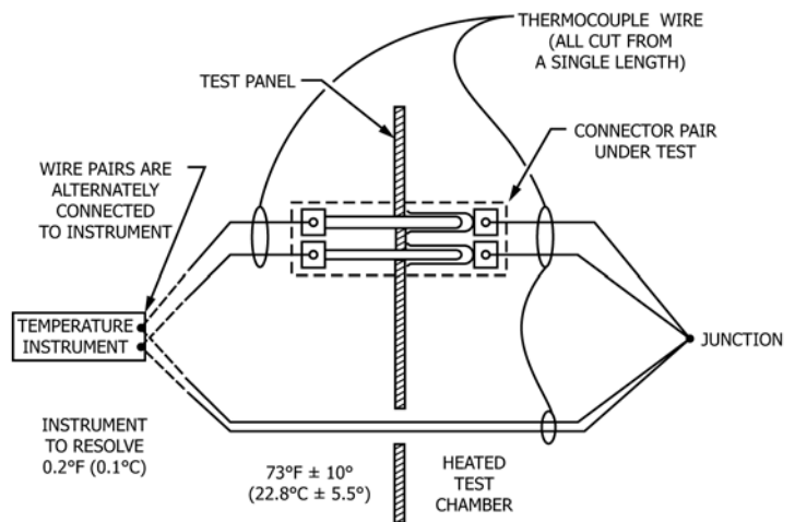
FIG. 4 Miniature Thermocouple Connector Test Circuit Diagram
