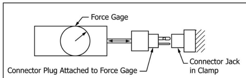
FIG. 6 Disengagement Force Test
