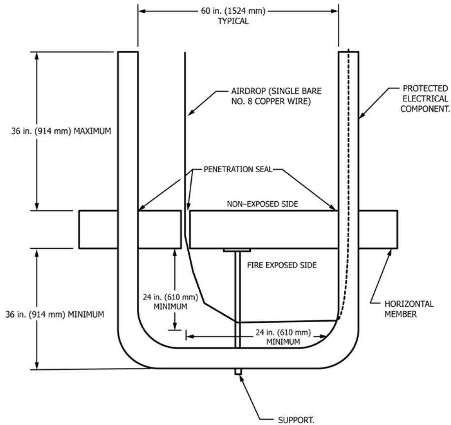
FIG. 6 Vertical and Horizontal Air Drop Assembly
