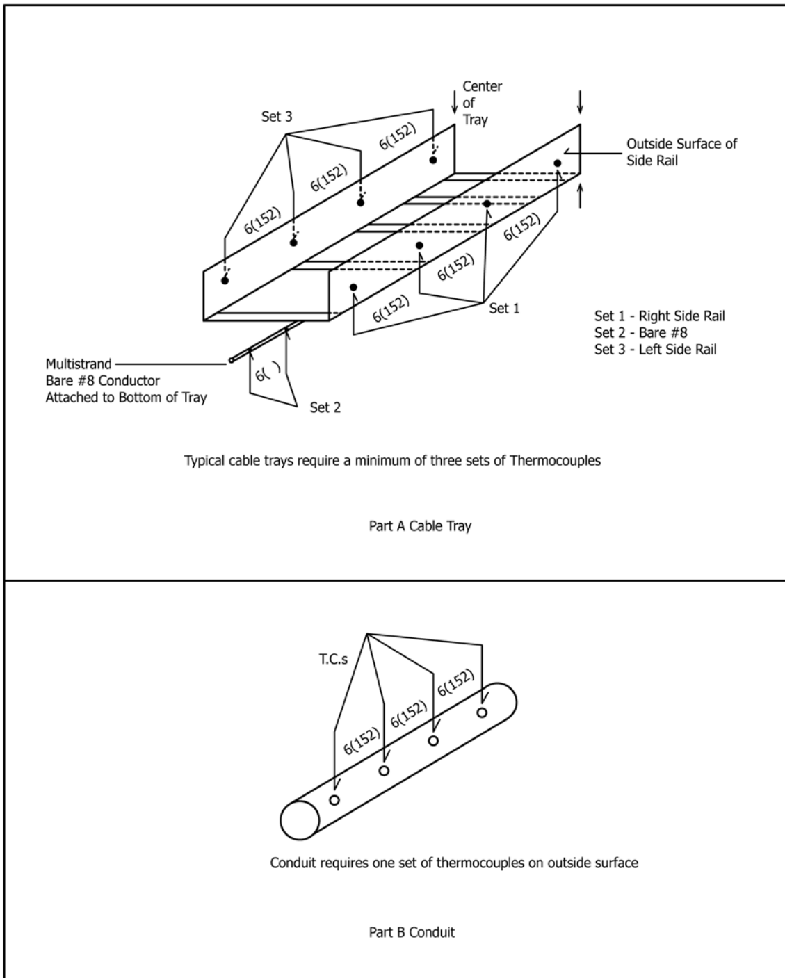
All dimensions are in inches All dimensions in ( ) are in millimeters FIG. 7 Specimen Thermocouples
