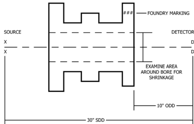
FIG. X1.1 Casting Radioscopic Examination Instruction Sheet (continued)
