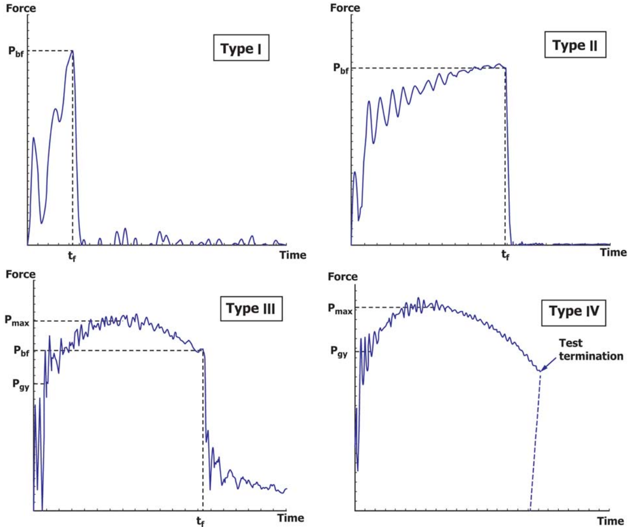
FIG. A17.1 Typical Force-time Diagrams (Schematic)
