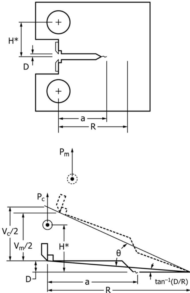
FIG. A2.3 Elastic Compliance Correction for Specimen Rotation
