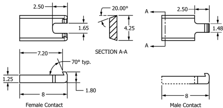
Contact Detail Contacts machined from Titanium 6Al-4V
