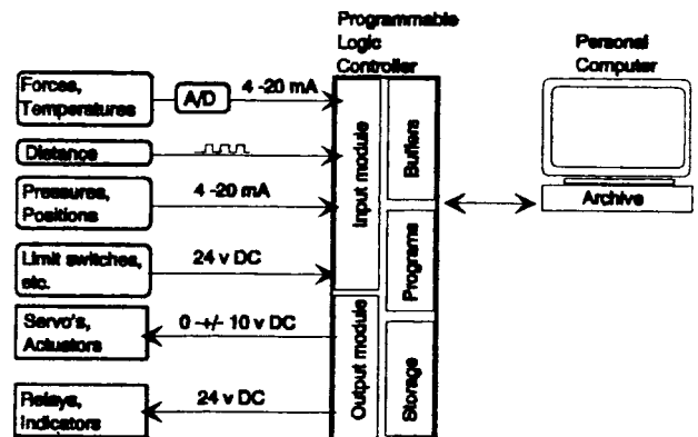
FIG. 3 Sample Instrumentation Scheme for Control and Measurements
