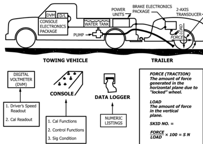
FIG. 1 Skid Measurement System
